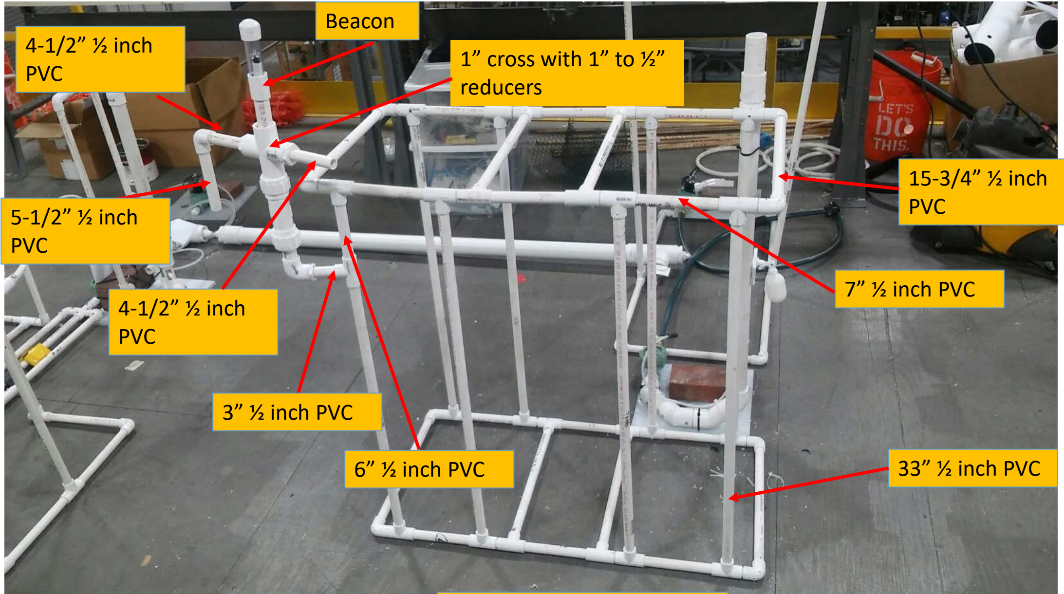
Vertical Tunnel and Beacon
